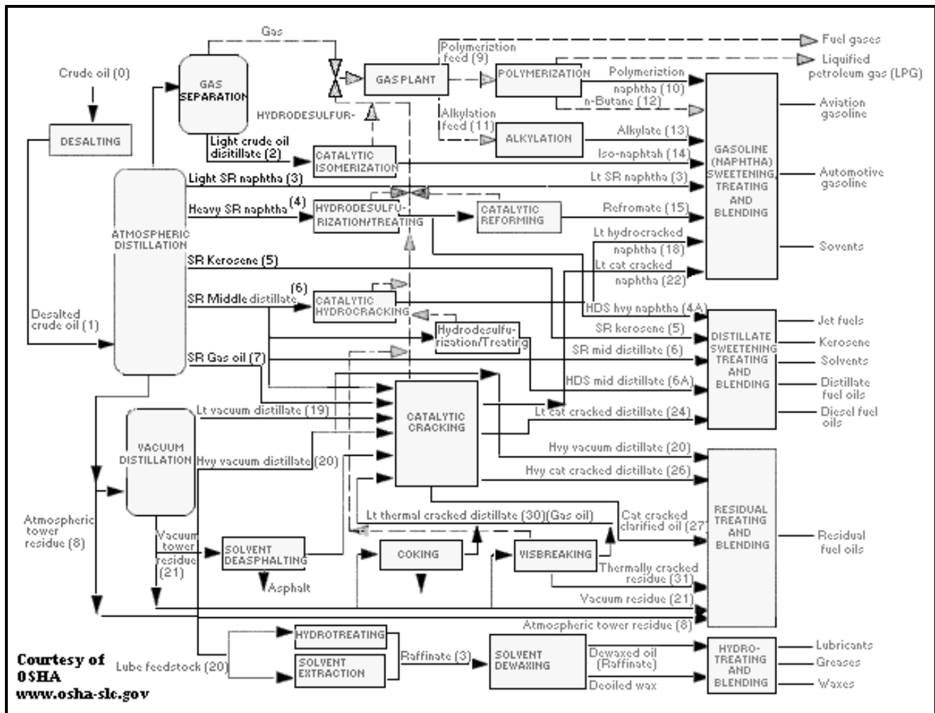
Exhibit 7: 理论（非常）杂炼油厂的流程简图
